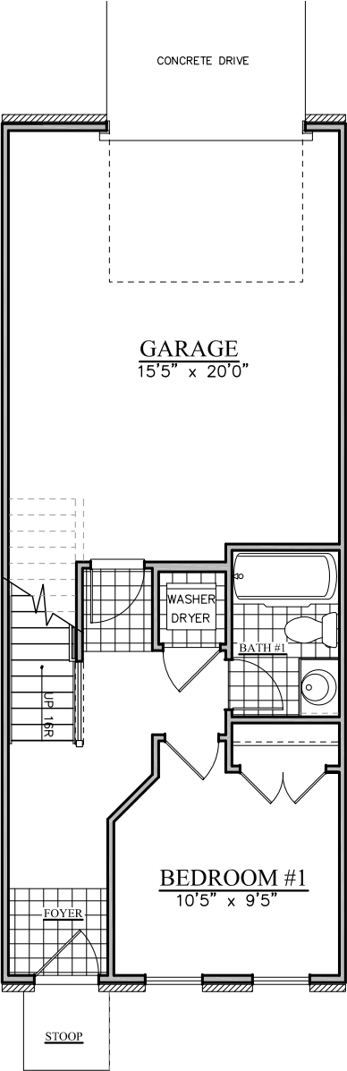
1ST FLOOR
